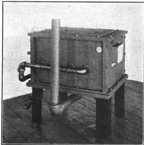
No. 10. Soft metal furnace used for tinning and galvanizing
